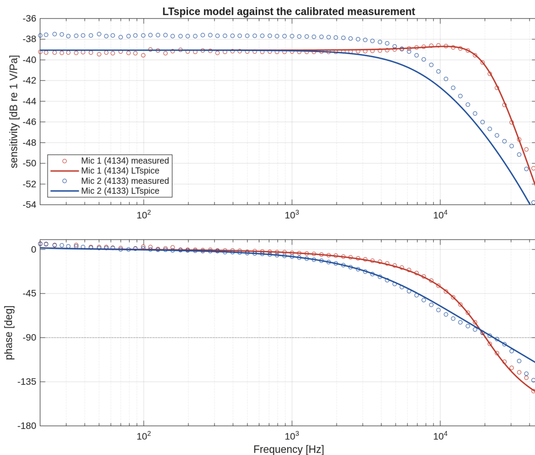
Figure 6: LTspice output (lines) against the calibrated measurement (circles), in absolute sensitivity. The LTspice source is entered with 180° phase, so no extra phase shift is needed.
